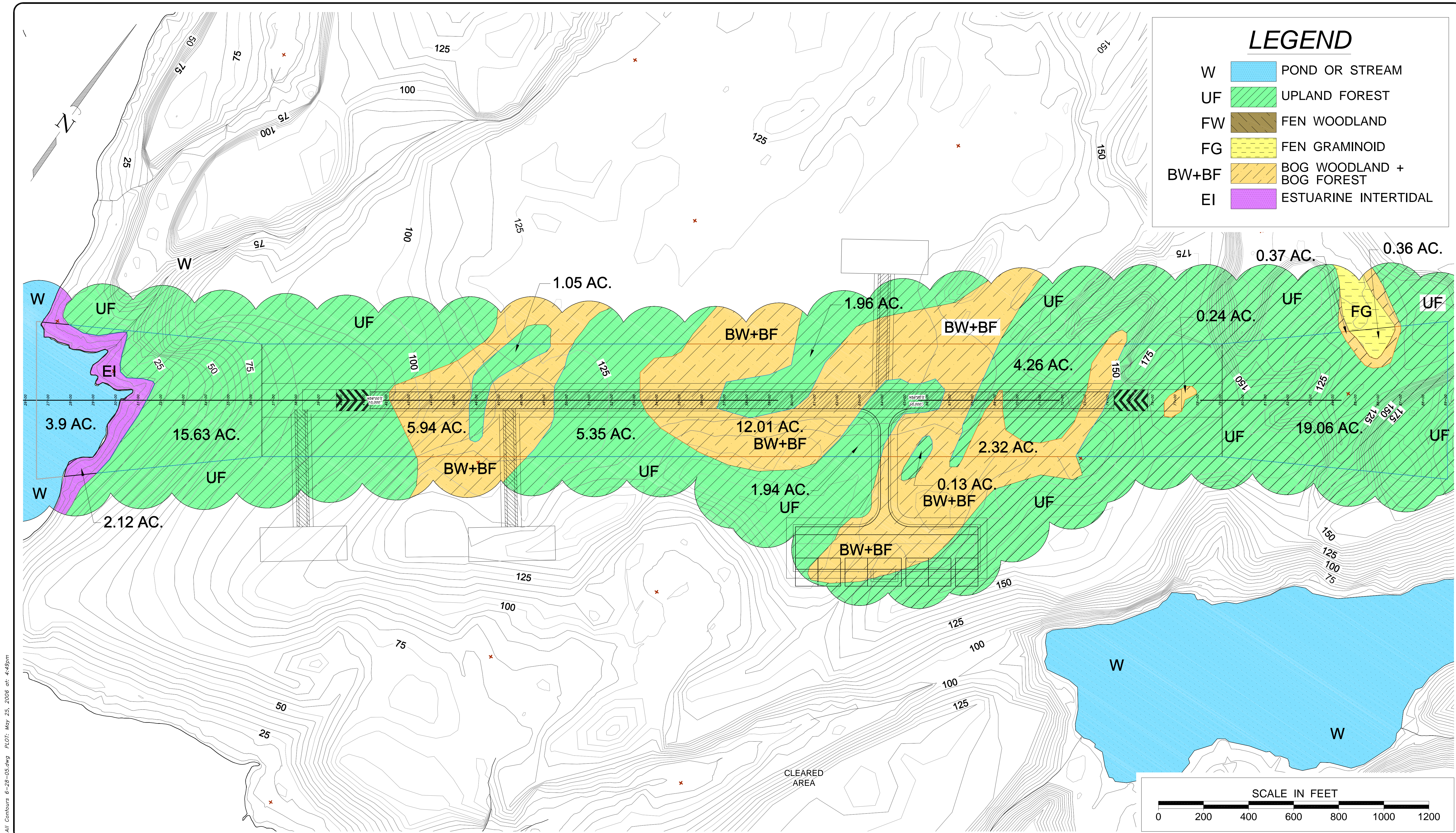
FIGURE 14. AIRPORT SITE WETLANDS
