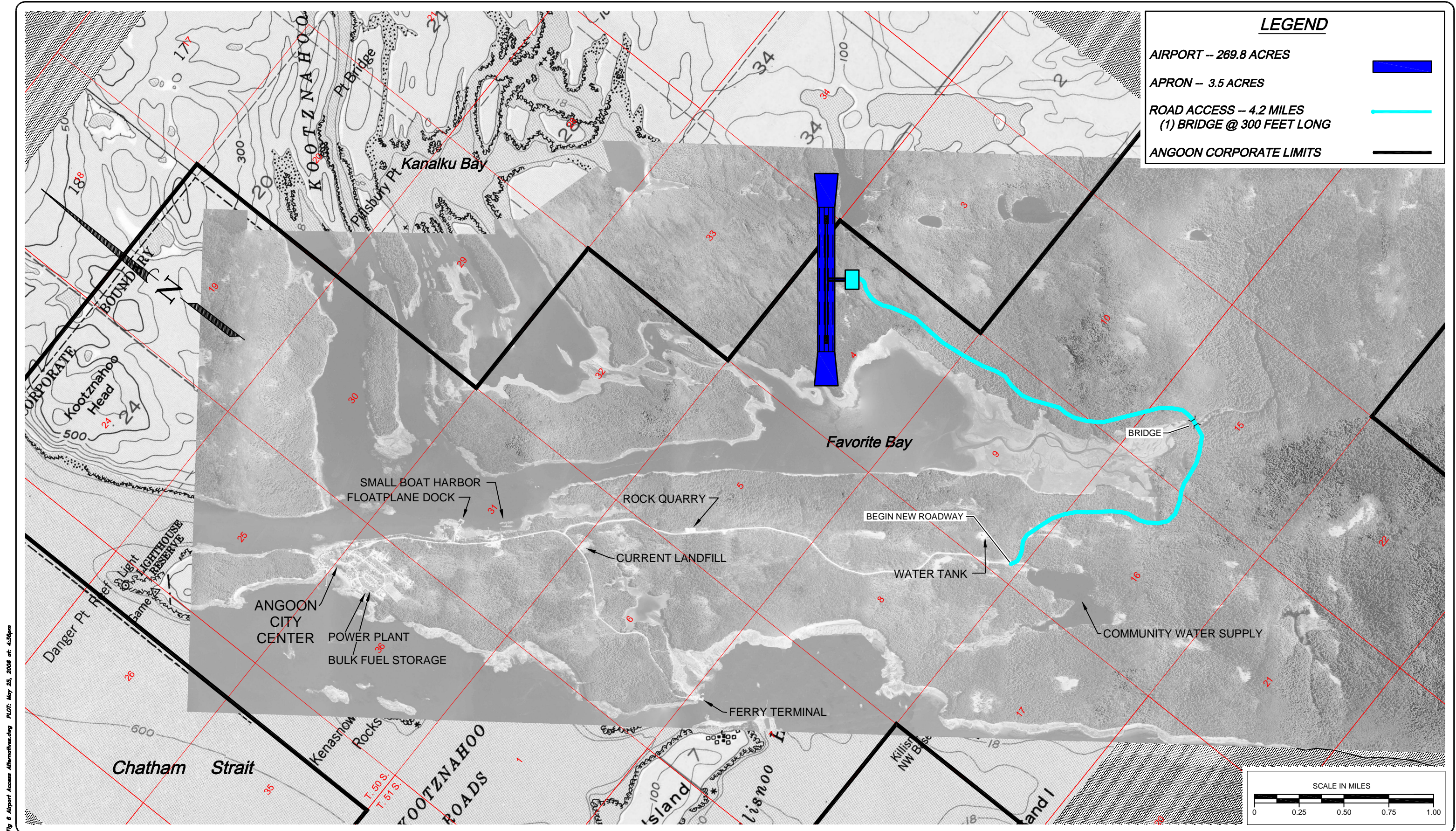
FIGURE 2. PROPOSED ANGOON AIRPORT SITE, APRON, AND ROAD ACCESS
